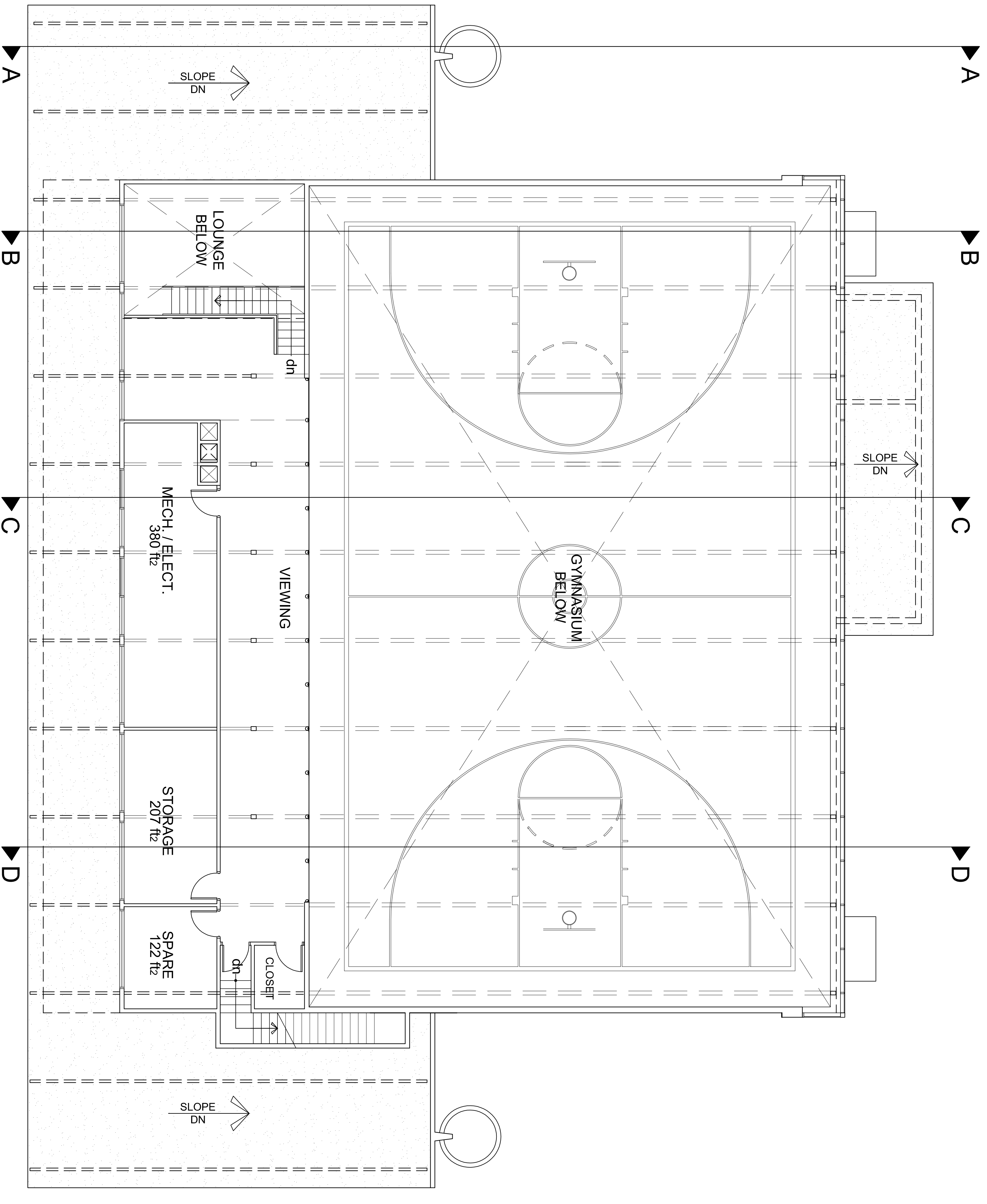
MEZZANINE FLOOR PLAN
